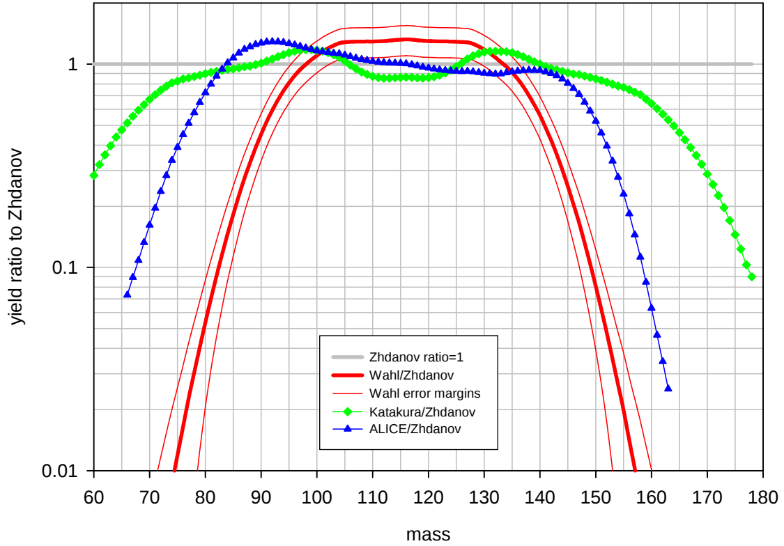
Benchmark B: ^{241}\text{Am} at 100 MeV, post neutron emission yield ratios to Zhdanovs data
